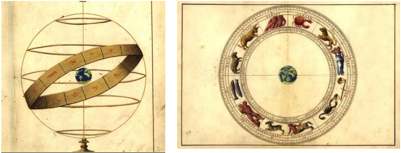
Figure 10: Two representations of the Zodiac around the Earth contained in a manuscript atlas by Battista Agnese from ca. 1544. 29 Images courtesy of the Library of Congress.
