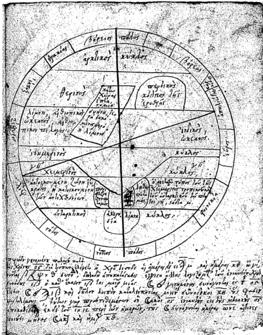
Figure 8: Greek cosmographical diagram with the Ecliptic drawn as a diagonal straight line (Oxford, Bodleian Library, Dept. of Oriental Collections, MS Marsh 42, fol. 4r /
