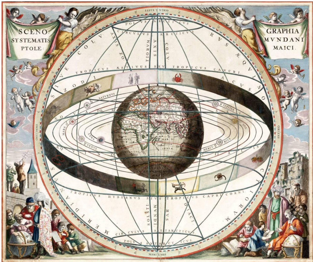
Figure 2: Cosmographical scheme showing the Earth in the center of the Universe and the Zodiac on the outer “sphere of stars,” according to Ptolemy’s theory; from Andreas Cellarius, Harmonia macrocosmica , ed. Johannes Janssonius (Amsterdam: 1660). Image courtesy of the National Library of Australia and Wikimedia Commons.
