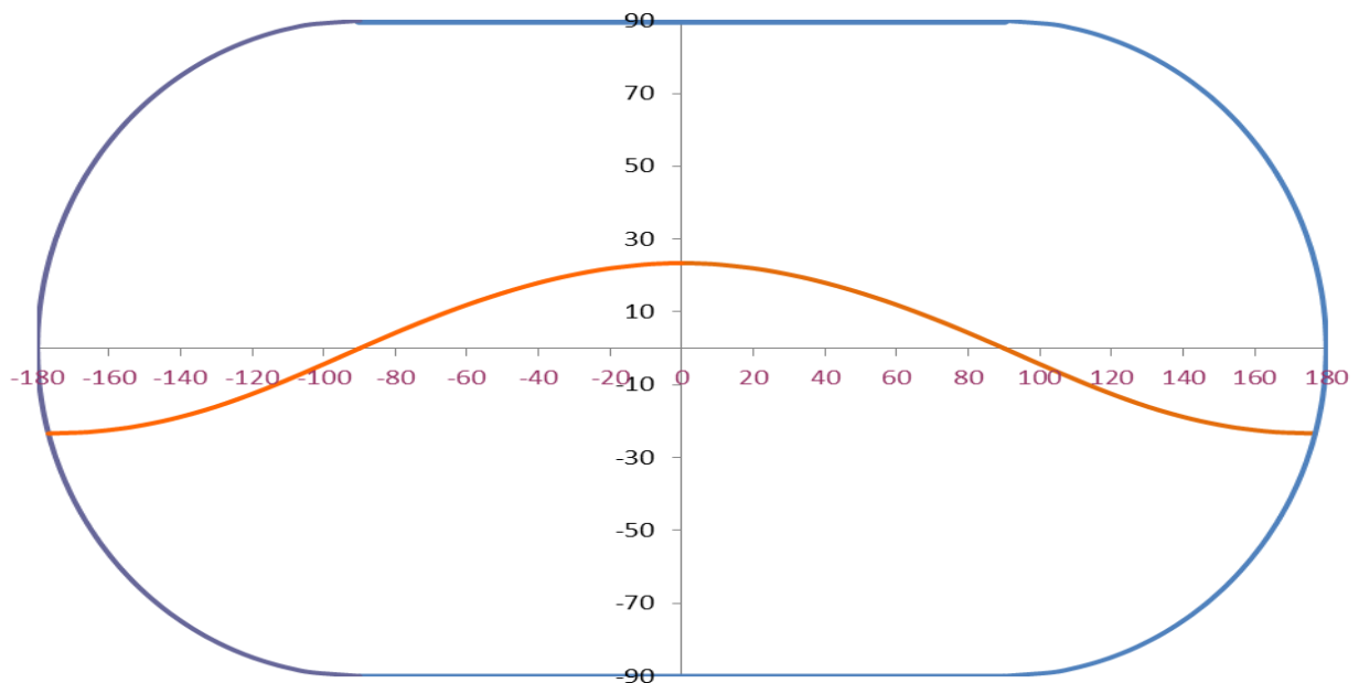
Figure 4: True shape of the Ecliptic in the Agnese Oval Projection.
