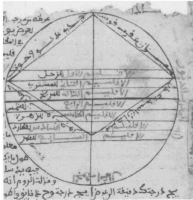
Figure 9: Cosmographical diagram from the Kitab al-Bad' wa-l-Ta'rikh (Bodleian Library, Oxford. Ms. Laud. Or. 317, fol. 7a). Copy dated 1569/70. Diameter of the original: 10.2 cm. Reproduced with permission from the Bodleian Library.
