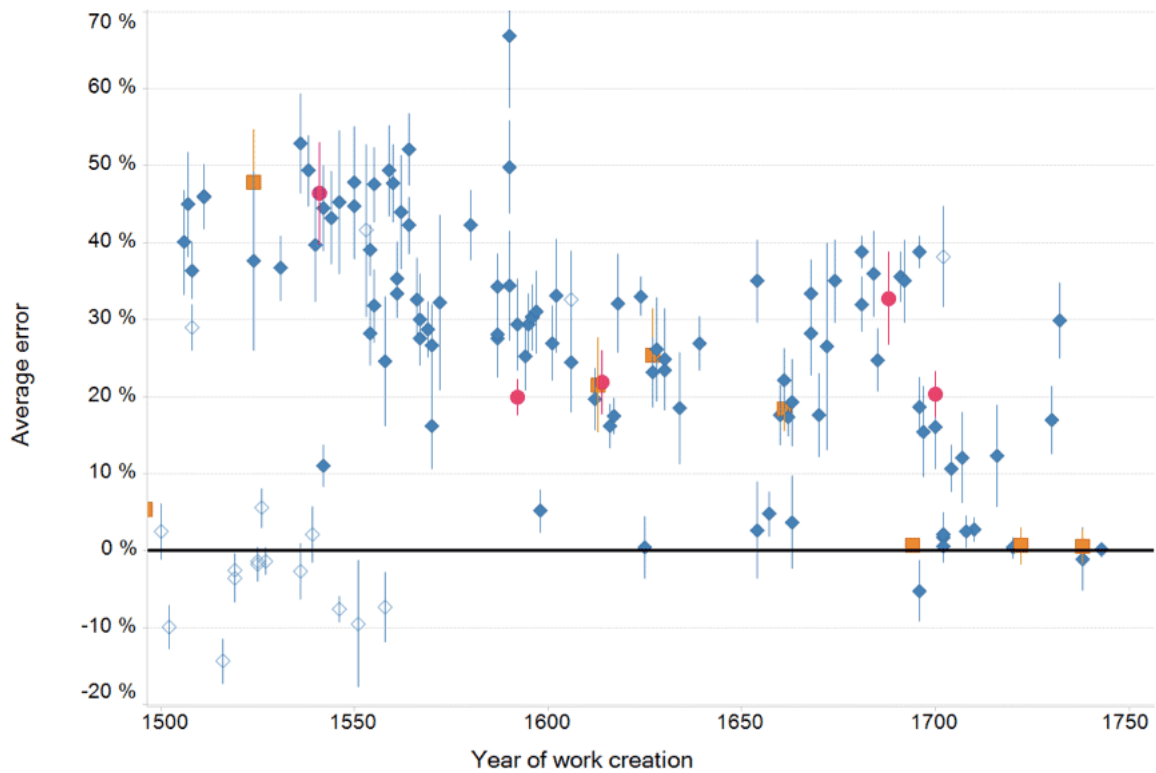
Figure 3: LongMed average error (dots) and standard deviation (error bars) vs year of creation of each cartographic work. Dot shapes and colors distinguish works by type: globes (pink circles), lists of coordinates (orange squares), graduated maps (filled blue diamonds) and maps with debatable projection (empty diamonds).
