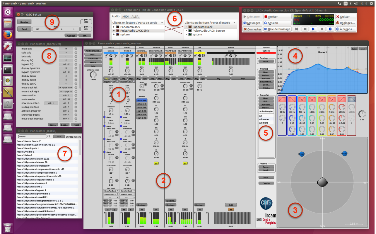
Figure 4: panoramix running in Ubuntu with Jack server (QJacketl) as audio pilot. ① Input tracks in the mixing console. ② Spatialization and reverberation busses. ③ Geometrical representation of the sound scene. ④ Parametric equalizer. ⑤ Group management. ⑥ Jack server and inter-application connections. ⑦ Status window: allows to inspect the current state of the engine and all parameters exposed to OSC messaging. ⑧ Shortcut window: allows to edit the key mappings. ⑨ OSC setup window: configure input and output port for remote communication.
