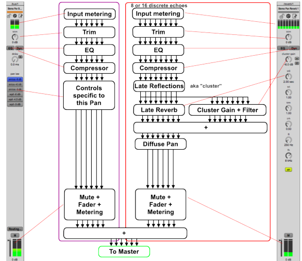
Figure 2: Anatomy of a bus: the purpose of a bus is twofold: it generates a late/diffuse reverberation tail (shared amongst multiple tracks for efficiency) and it provides control over the spatialization rendering. The lefthand side (violet frame) depicts the panning bus; the righthand side (red frame) represents the late reverb bus.
