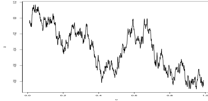
FIG 2. Graph of the chosen function a_1^{(0.5)} .
