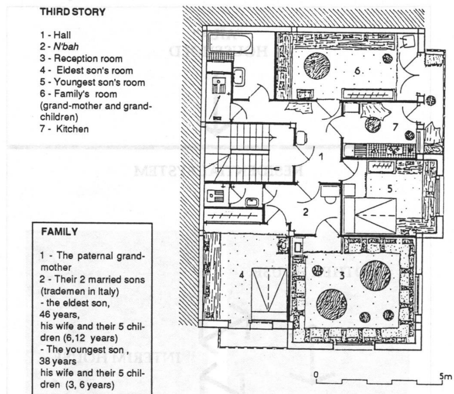
Fig. 2 Plan of a house noticed in Khouribga, Morocco. A property which is shared by two brothers who emigrated to Italy and left their family in the country of departure.
