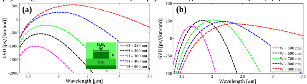
Fig. 1. GVD profiles of strained Si waveguides with different (a) height – H and width of 700 nm, (b) widths – W and height of 400 nm.
