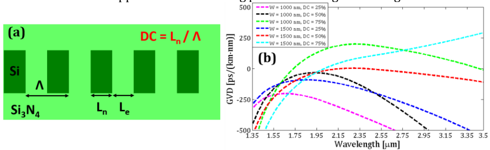
Fig. 2. (a) 2-D schematics of the SWG waveguide. (b) GVD profiles of the strained metamaterial waveguides for different waveguide widths and SWG geometries.
