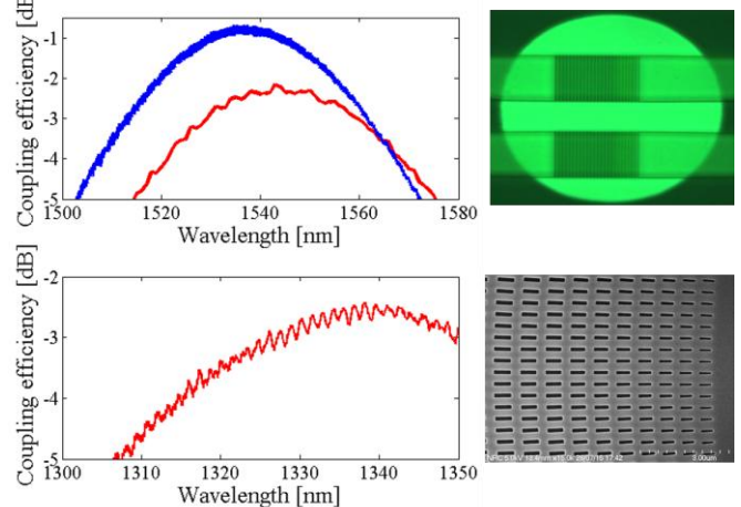
Fig. 1 Measured coupling efficiencies as a function of wavelength of single-etch apodized grating couplers, with and without metal reflector underneath. Optical micrograph and SEM images of fabricated structures.
