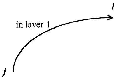
Graph for \mathbf{W}^{(1)} = \mathbf{W}_1 * \mathbf{W}^{(0)} = \mathbf{W}_1
