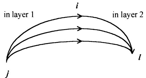
Graph for \mathbf{W}^{(2)} = \mathbf{W}_1 * \mathbf{W}^{(1)}
