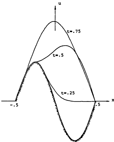
Figure 9 Obstacle u = \phi(x) = -\sin \pi x \cdot \cos \pi x String initially at rest on the obstacle
