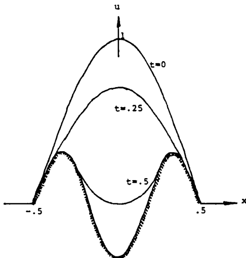
Figure 12 Obstacle u = \Phi(x) = -\frac{1}{3}\cos\pi x
