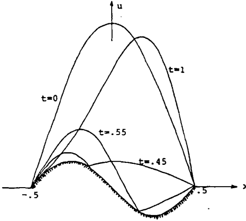
Figure 5 Obstacle u = \Phi(x) = -\frac{1}{3} \sin \pi x \cdot \cos \pi x
