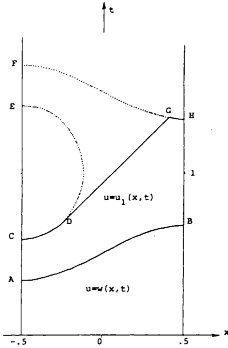
Figure 4 Obstacle u = \Phi(x) = -\tan \frac{\theta}{2} \cdot \sin \pi x \cdot \cos \pi x
