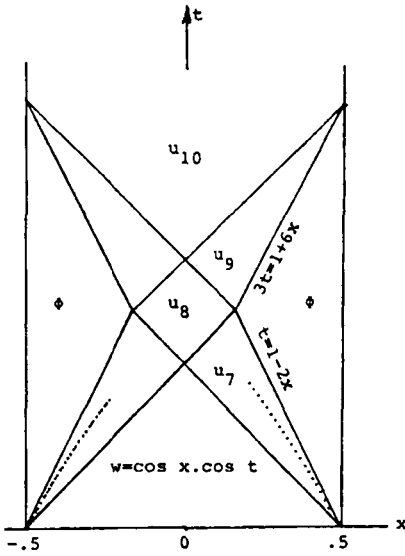
Figure 11 Obstacle u = \Phi(x) = -\frac{1}{3} \cos 3\pi x String u(x,0) = \cos \pi x, \frac{\partial u}{\partial t} = 0 Periodic motion: period T = \frac{4}{3}
