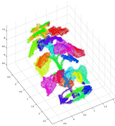
Figure 3: Result of K-means algorithm with k=25
