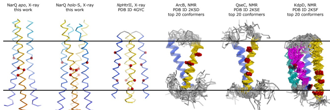
1 2 Figure S5. Comparison of the experimentally determined structures of TCS TM domains. In each case, the N- 3 terminal \alpha -helix TM1 is shown in blue and the C-terminal one is shown in yellow. Glycine and proline residues of 4 the TM helices are shown with red spheres. There are generally more glycine and proline residues in the last TM 5 helix of the histidine kinases. The scale is the same for all of the proteins. X-ray structure of NpHtrII (28) 6 is aligned to ligand-bound NarQ structure using the positions of the HAMP-domain proximal residues that are similar, 7 opposite to the positions of the residues in the middle of the membrane and at the periplasmic side. Since there is no 8 sequence similarity between the TM domains, NMR structures of ArcB, QseC and KdpD (15) are aligned to the 9 NarQ structure so that their helices are roughly at the same positions relative to the membrane. Structural 10 comparison with ArcB, QseC and KdpD is hampered since the structures are monomeric and information about the 11 dimerization interfaces is lacking (15). It is not clear whether the ArcB and QseC fragments are in the correct 12 physiological state. In the KdpD structure, presence of the additional TM helices (TM2 and TM3, cyan and 13 magenta) probably ensures correct folding of the TM domain and proper orientations of the N-terminal and C- 14 terminal helices.
