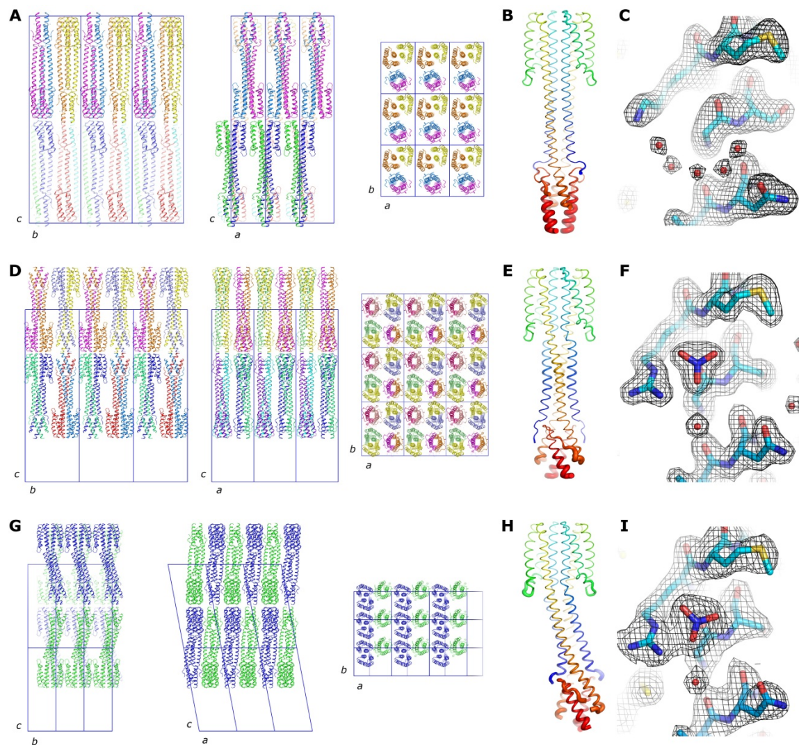
Figure S2. Crystallographic details. (A-C) Data for the space group I 2 1 2 1 2 (symmetric apo state structure). (D-F) Data for the space group F222 (symmetric holo state structure). (G-I) Data for the space group P2 (asymmetric holo state structure). (A, D, G) Crystal packing. The NarQ dimers pack in layers, as is typical for Type I membrane protein crystals, obtained through in meso crystallization. (B, E, H) Relative distributions of the B-factor values. The scale in each drawing is different. In each space group, the membrane-distal parts of the HAMP domain are notably disordered. (C, F, I) Example of the electron density maps for the chain A residues around the ligand binding site. Weighted 2F o -F c electron density maps are contoured at the level of 1.5 σ.
