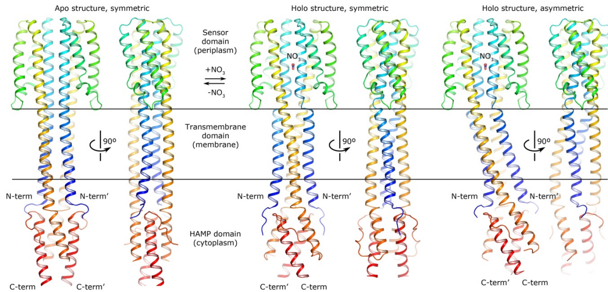
5 Figure 1. Overall structure of the crystallized NarQ fragment in apo and holo states. The 6 protein is observed as a symmetric dimer in both the apo and holo-S states in the space groups 7 I2_12_12_1 and F222, respectively, and as an asymmetric dimer in holo-A state in the space group 8 P2. Termini of the second protomer are denoted with primes. The crystallized fragment 9 comprises the transmembrane domain (helices TM1 and TM2), the periplasmic sensor domain 10 (helices H1-H4) with the nitrate ion binding at the dimerization interface, and the intracellular 11 HAMP domain (helices AS1 and AS2). The structures are aligned by sensor domains. 12 Hydrophobic membrane boundaries (black) were calculated using the OPM server (67) with the 13 symmetric ligand-bound structure as a template.
