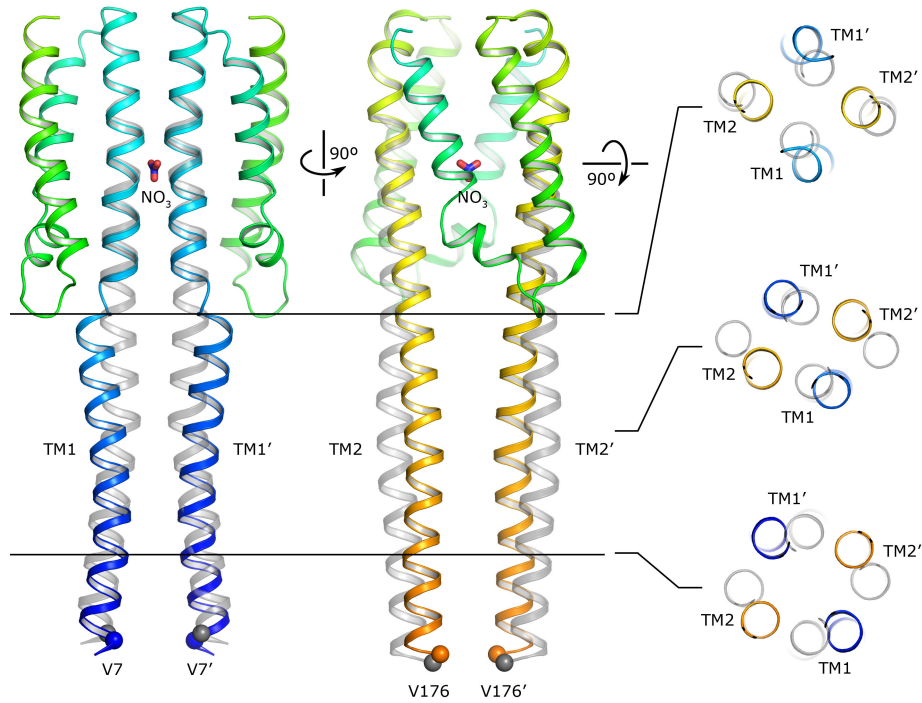
1 2 Figure 2. Signaling-associated conformational changes in the NarQ TM domain. 3 Superposition of the apo state structure (grey) and symmetric holo state structure (colored) is 4 shown. Left, changes in conformation of the helix TM1. Middle, changes in conformation of the 5 helix TM2. Right, changes in the arrangement of the TM helices. C_{\alpha} atom positions of the 6 residues from CC layer 9 are marked with the spheres to highlight the displacements in the 7 direction perpendicular to the membrane. The structures are aligned by the sensor domains. 8
