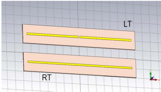
Fig. 4. Simulation of two tags: gain and impedance are measured at the Listener Tag (LT), while the Reader Tag (RT) could switch between Open Circuit and Short Circuit (here Short Circuit).
