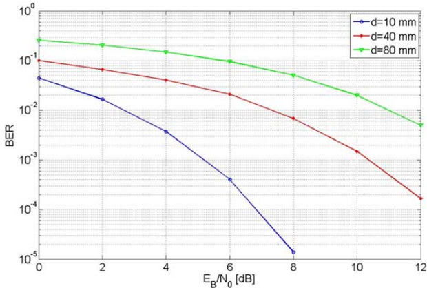
Fig. 8. BER variation with respect to the signal to noise ratio for different distances between RT and LT tags. The source position is at \theta = 45 degrees.
