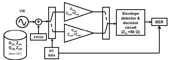
Fig. 6. Global scheme of the system-level simulations.
