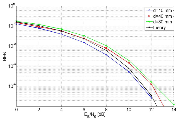
Fig. 7. BER variation with respect to the signal to noise ratio for different distances between RT and LT tags. The source position is at \theta = 0 degrees.
