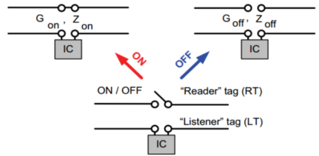
Fig. 2. Two states of the tag-to-tag communication: ON and OFF corresponding to the reader tag switching between an open circuit and a short circuit [10].
