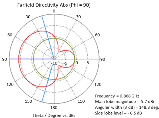
Fig. 5. Example of radiation pattern obtained when simulating the two near field coupled tags.
