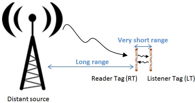
Fig. 1. Global principle of tag-to-tag communication.
