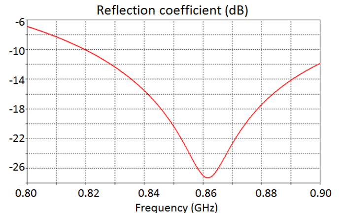
Fig. 3. Reflection coefficient (i.e., S_{11} parameter) of the simulated dipole without coupling with another tag.
