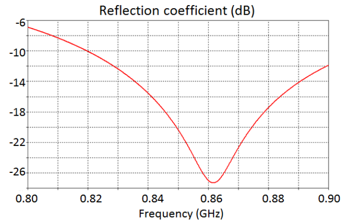
Fig. 3. Reflection coefficient (i.e., S_{11} parameter) of the simulated dipole without coupling with another tag.
