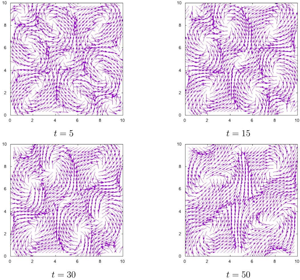
FIGURE 2. Taylor-Green vortex problem. Numerical solution \mathbf{v}_f at time t = 5 , t = 15 , t = 30 and t = 50 .
