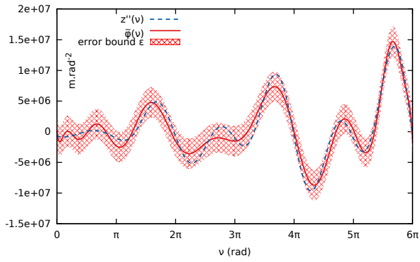
(c) Rigorous approximation \tilde{\varphi} of degree n = 18 of z'' , over [0, 6\pi] and for e = 0.5
