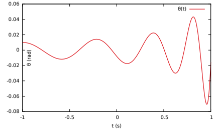
(c) Damped oscillations of the pendulum obtained for \ell_0 = 0.1 and \zeta = 0.9 (d) Diverging oscillations of the pendulum obtained for \ell_0 = 0.1 and \zeta = -0.9
