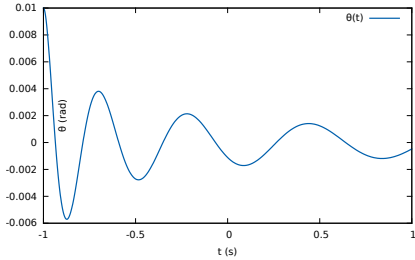
(c) Damped oscillations of the pendulum obtained for \ell_0 = 0.1 and \zeta = 0.9 (d) Diverging oscillations of the pendulum obtained for \ell_0 = 0.1 and \zeta = -0.9
