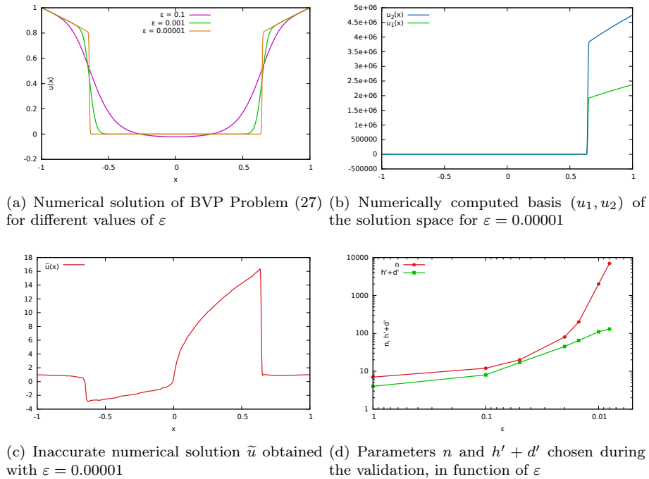
Figure 6: Validation process for the boundary layer problem
