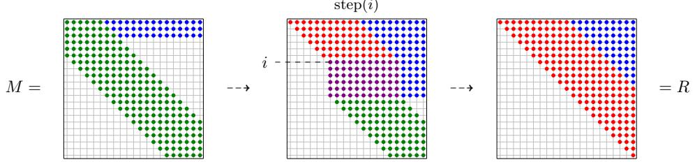
Figure 2: Step 1 of Olver and Townsend's algorithm
