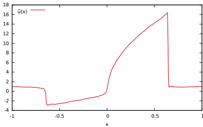
(c) Inaccurate numerical solution \tilde{u} obtained with \varepsilon = 0.00001
