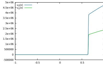
(b) Basis (u_1, u_2) of the solution space for \varepsilon = 0.00001
