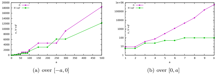
Figure 4: Parameters n and h' + d' chosen during the validation, in function of a
