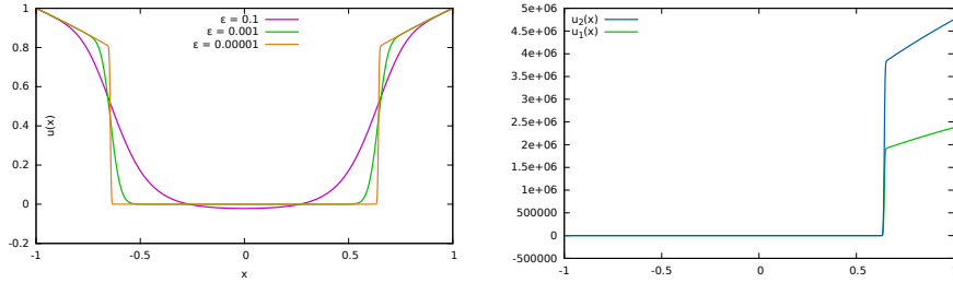
(a) Solution of BVP Problem (26) for different values of \varepsilon (b) Basis (u_1, u_2) of the solution space for \varepsilon = 0.00001
