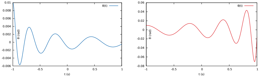
(c) Damped oscillations of the pendulum obtained for l_0 = 0.1 and \zeta = 0.9 (d) Diverging oscillations of the pendulum obtained for l_0 = 0.1 and \zeta = -0.9
