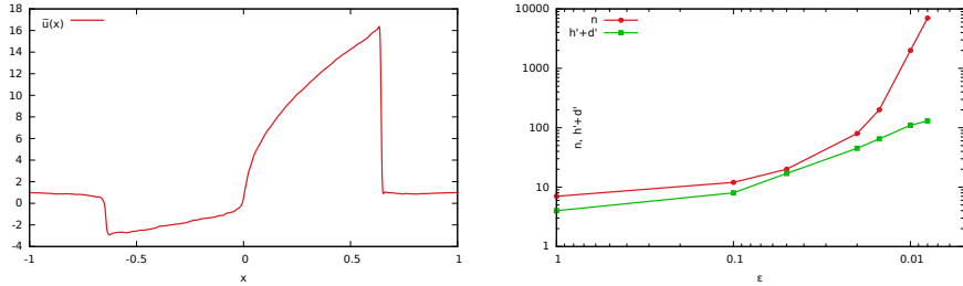
(c) Inaccurate numerical solution \tilde{u} obtained with \varepsilon = 0.00001 (d) Parameters n and h' + d' chosen during the validation, in function of \varepsilon
