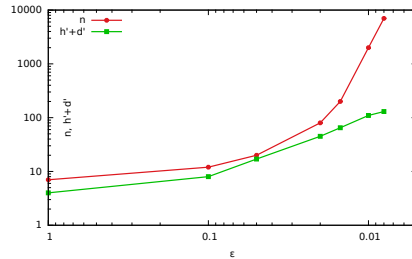
(d) Parameters n and h' + d' chosen during the validation, in function of \varepsilon
