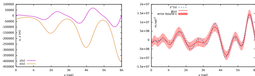
(a) Exact representation of x(\nu) and z(\nu) for \nu \in [\nu_0, \nu_f] (b) Rigorous approximation \tilde{\varphi} of degree n = 18 of z''
