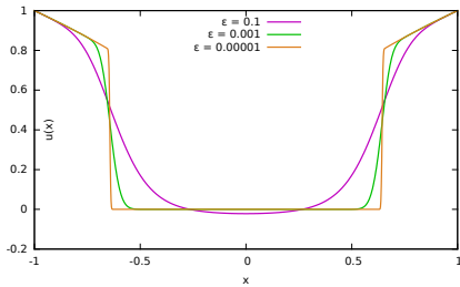
(a) Solution of BVP Problem (26) for different values of \varepsilon
