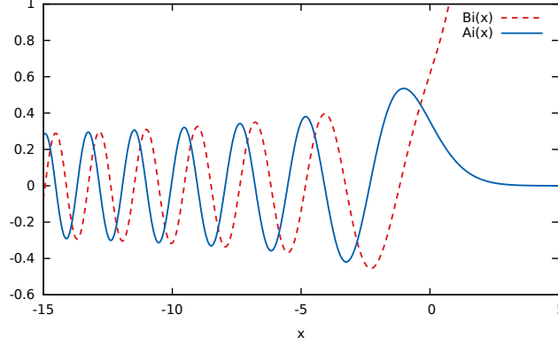
Figure 3: Airy functions of the first and second kinds
