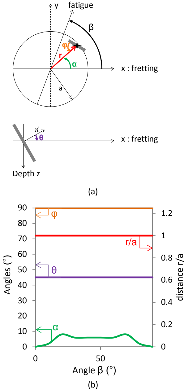
Figure 14: (a) Definition of parameters r , \alpha , \theta and \varphi for crack nucleation localization and critical plane orientation. (b) Evolution of the four parameters as functions of \beta . ( R=200\text{mm} , P=5000\text{N} , \sigma_{F,\text{max}}=400\text{MPa} , R_\sigma=0.8 ).
