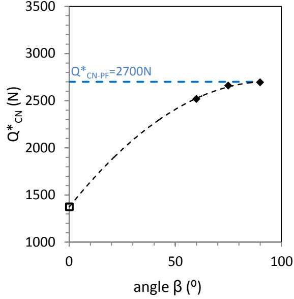
Figure 9: Crack nucleation conditions as functions of angle \beta ( R=200\text{mm} , P=5000\text{N} , \sigma_{F,\text{max}}=400\text{MPa} , R_\sigma=0.8 , 10^6 cycles). ( \blacklozenge ) Non collinear FF crack nucleation conditions (NCCF test: centroid fatigue stress \rightarrow no eccentricity); ( \blacksquare ) Collinear fretting fatigue crack nucleation condition (FF test: eccentricity).
