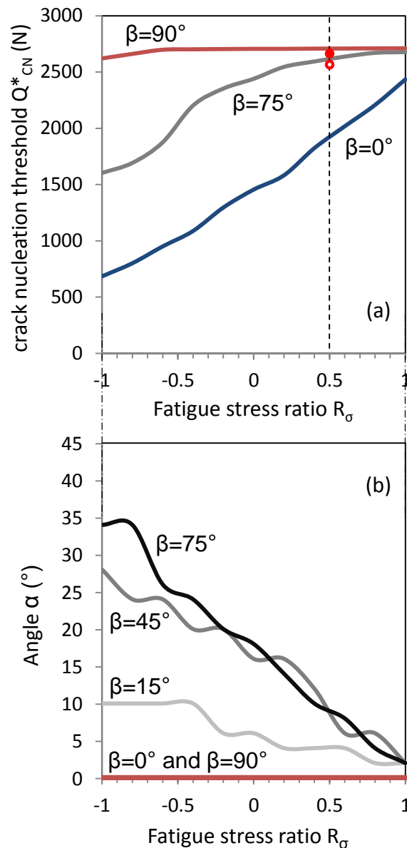
Figure 15: (a) evolution of crack nucleation threshold Q_{CN}^* as a function of the fatigue stress ratio R_\sigma .
