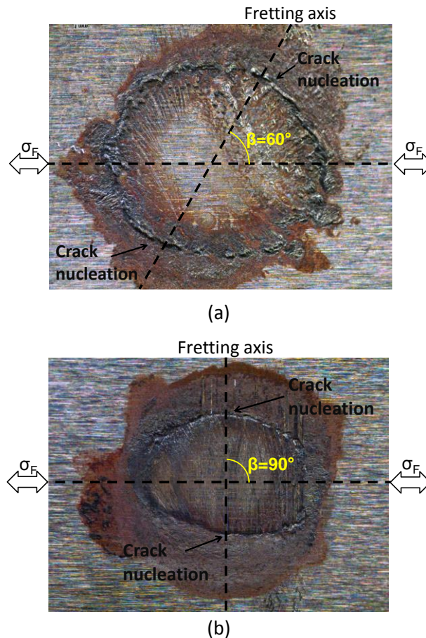
Figure 7: Fretting scars in multiaxial fretting fatigue after 10^6 cycles. (a) \beta=60^\circ , Q^*=2700N ; (b) \beta=90^\circ , Q^*=3100N . ( R=200mm , P=5000N , \sigma_{F,max}=400MPa , R_\sigma=0.8 , 10^6 cycles).
