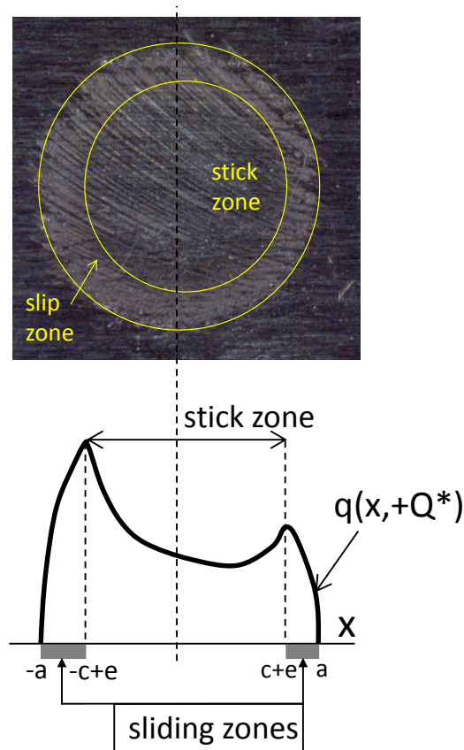
Figure 5: Eccentricity in collinear fretting fatigue
