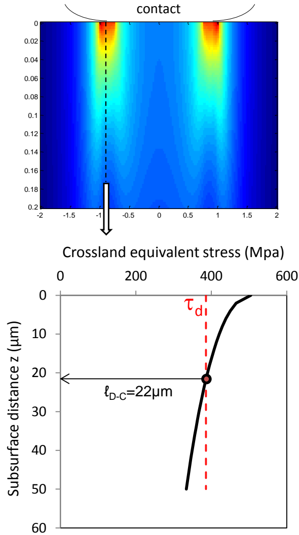
Figure 11: Identification of critical distance l_{D-C} from subsurface Crossland distribution ( R=200\text{mm} , P=5000\text{N} , Q^*=2700\text{N} ).
