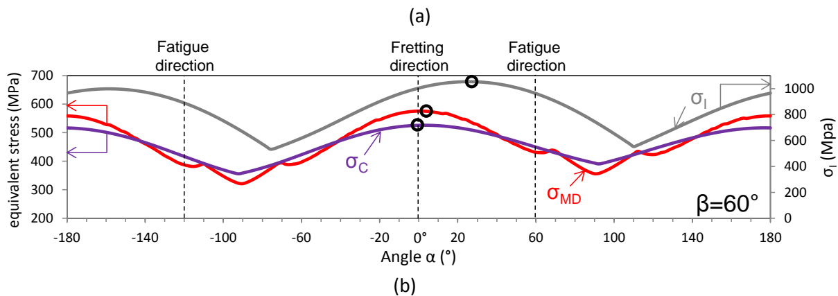
Figure 10: (a) XY mapping of \sigma_1 , Crossland, Mc Diarmid as function of fretting fatigue loading and localization of maximum cracking risk. (b) \sigma_1 , Crossland, Mc Diarmid evolution along the contact border for \beta=60^\circ . ( R=200\text{mm} , P=5000\text{N} , Q^*_{CN} , \sigma_{F,max}=400\text{MPa} , R_0=0.8 , 10^6 cycles).
