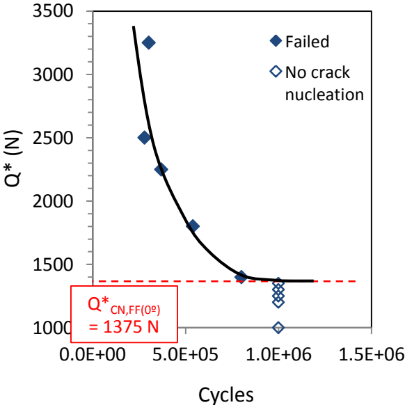
Figure 6: Identification of crack nucleation condition under collinear fretting fatigue loading \beta=0^\circ ( R=200 mm, P=5000 N, \sigma_{F,max}=400 MPa, R_\sigma=0.8 , 10^6 cycles).
