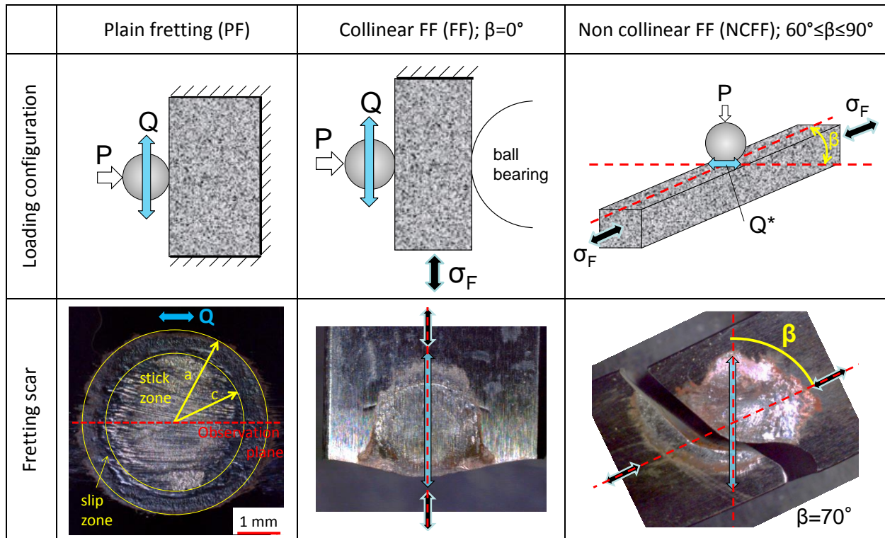
Figure 2: Loading configurations and related fretting scars for the three test configurations: plain fretting, conventional collinear fretting fatigue and on collinear fretting fatigue. ( R=200\text{mm} , P=5000\text{N} , Q^*=2700\text{N} , \sigma_{F,\text{max}}=400\text{MPa} , R_\sigma=0.8 , 10^6 cycles). \longleftrightarrow : Fretting loading direction; \blackleftarrow\blackrightarrow : fatigue loading direction.
