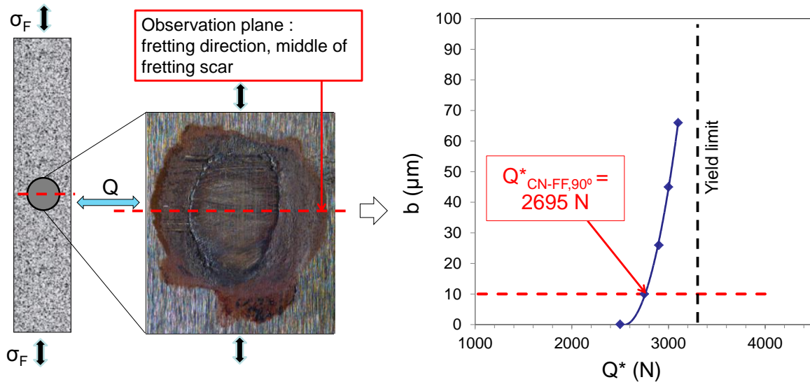
Figure 8: Illustration of the methodology used to identify the crack nucleation of non collinear fretting fatigue experiments ( R=200\text{mm} , P=5000\text{N} , \sigma_{F,\text{max}}=400\text{MPa} , R_\sigma=0.8 , 10^6 cycles, \beta=90^\circ )
