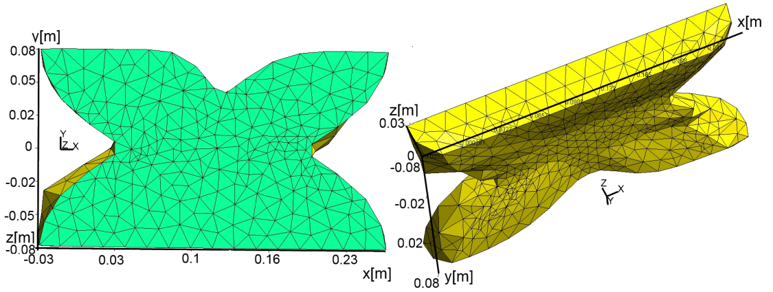
Figure 9: Optimized sole for the case 2-Rot: ZMP trajectory illustrated in Fig. 6, material neoprene and w = 1000 in the cost function (1)
