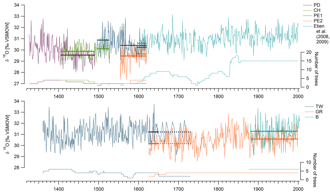
Figure 4. Cohort offsets. Top: The \delta^{18}\text{O}_C series for different tree cohorts from Fontainebleau. Bottom: the \delta^{18}\text{O}_C series for living tree cohorts (B and GR), and timber wood (TW) from Angoulême. Horizontal lines indicate the mean of each series for the period of overlap. TW samples have been measured every 5th year only in the period covered by the dotted line.
