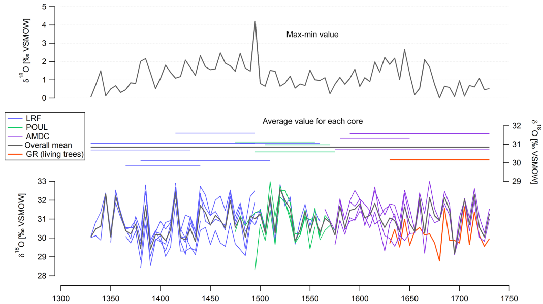
Figure 3. Inter-tree comparison. Bottom: \delta^{18}\text{O}_C measured every 5th year for individual timber cores from different buildings in Angoulême (LRF, POUL, and AMDC). The orange line shows the \delta^{18}\text{O} of living trees (GR). Middle: time spans and average \delta^{18}\text{O} values for the respective cores. The thick gray line is the mean \delta^{18}\text{O} of all timber cores over the whole period. Top: range of measured values for each year (maximum minus minimum value).
