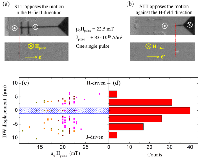
FIG. 4. STT effect on DW motion for strong J_{\text{pulse}} > 33 \times 10^{10} \text{ A/m}^2 . (a) and (b) are DW displacement observations for combined \mu_0 H_{\text{pulse}} = 22.5 \text{ mT} and J_{\text{pulse}} = +33 \times 10^{10} \text{ A/m}^2 excitations, which lead to movements in two opposite directions. Cases (a) and (b) are respectively called H -driven and J -driven. Each case is depicted by two MOKE pictures: the upper one represents the DW position in the wire before pulses with magnetic states of each domain shown (white symbols); the bottom one is the DW position after the combined H_{\text{pulse}} and J_{\text{pulse}} excitations (both displayed in yellow). The black magnetic contrast corresponds to the H -driven DW motion, the white one to the J -driven case. (c) Plot of all experimental data points measured for DW displacement versus \mu_0 H_{\text{pulse}} for various J_{\text{pulse}} (magenta: 33 , brown: 37 , orange: 41 , and dark yellow: 45 \times 10^{10} \text{ A/m}^2 ). Positive displacement is for H -driven, the negative one for J -driven. The blue shaded region represents the range of DW pinning or automotion (points located in this region correspond to several measurements). (d) Bar graph of the DW displacement. The statistics was built from all experimental data from (c) without taking into account the value of the current.
