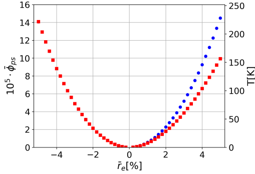
Figure 4. Depth of the three local potential minima versus a single rod displacement (same sign convention as in Fig. 3). The blue circles correspond to the minimum aligned with the displaced rod and the centre of the trap, the red squares to the two other minima. For \bar{r}_e < 0 , values are too close to be distinguished. Two scales for the pseudo-potential are used. Left y -axis : \bar{\phi}_{ps} . Right y -axis : Q\phi_{ps}/k_B (K), the scaling factor is computed with our experimental parameters ( \text{Ca}^+ , r_0 = 3.83 mm, \Omega/2\pi = 3.3 MHz and V_{rf} = 300 V).
