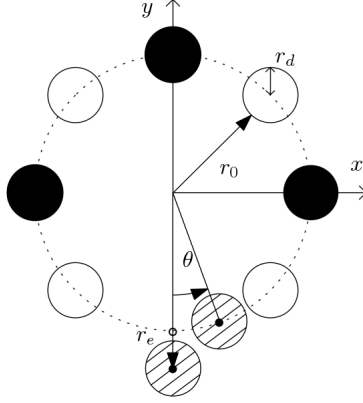
Figure 2. Scheme in the radial plane of the electrodes of a linear octupole trap. Black and white rods are polarised by \pm V_{rf} voltages. The dash-filled circle corresponds to the displaced rod and the relevant radii and angle are drawn.
