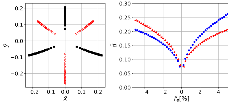
Figure 3. Left : Position of the local potential minima for displacement \bar{r}_e ranging from 0.2 to 5% of the rod located on the negative y -axis. The smallest displacement gives rise to the closest minima to the trap centre. The filled squares correspond to a rod displaced towards the trap centre, the open circles to a rod displaced away from the centre. Right : Distance of the three minima to the trap centre as a function of the normalized rod displacement. The blue circles correspond to the minimum on the y -axis and the red triangles to the other two minima. As a convention, \bar{r}_e > 0 stands for a rod at a radius larger than r_0 , \bar{r}_e < 0 for a rod closer to the centre.
