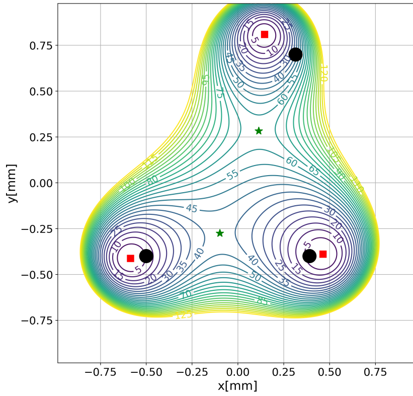
Figure 6. Pseudo-potential given by CPO for the best agreement with the experimentally determined local minima (black circles) out of the 2000 test cases. The red squares represent the minima of the best agreement, and the green stars the saddle points used to compute the potential. The numerical values in the iso-lines correspond to a temperature in Kelvin when using parameters of our experimental set-up. See text for details.
