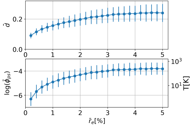
Figure 5. Random radial variation of all trap rods. Top : Mean value of the distance of the minima to the trap centre versus the relative distance of the rods to their nominal position r_e/r_0 . Bottom, left scale : mean of normalised potential depth \log \bar{\phi}_{ps} versus r_e/r_0 . Bottom, right scale : mean potential depth in temperature units Q\phi_{ps}/k_B (K), the scaling factor is computed with our experimental parameters ( \text{Ca}^+ , r_0 = 3.83 mm, \Omega/2\pi = 3.3 MHz and V_{rf} = 300 V).
