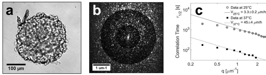
Figure 6. Speckle fluctuation analysis on 3D multicellular aggregates. (a) Bright-field image of a spherical aggregate of radius R \simeq 100 \mu\text{m} . (b) Speckle pattern generated by the aggregate. To avoid saturation, shorter exposure times are used at small q . (c) Cell dynamics in 3D aggregates. Correlation times are computed both at physiological ( 37^\circ\text{C} ) and at low ( 25^\circ\text{C} ) temperature. At 25^\circ\text{C} (empty circles) the mean speed is \bar{v}_{25^\circ} = 3.3 \pm 0.2 \mu\text{m/h} . At 37^\circ\text{C} (filled squares) we measure \bar{v}_{37^\circ} = 45 \pm 4 \mu\text{m/h} .
