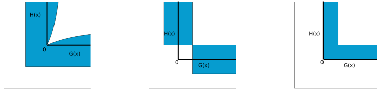
Fig. 1: The feasible set of the butterfly relaxation, the approximation from [17] and the relaxation from [19].
