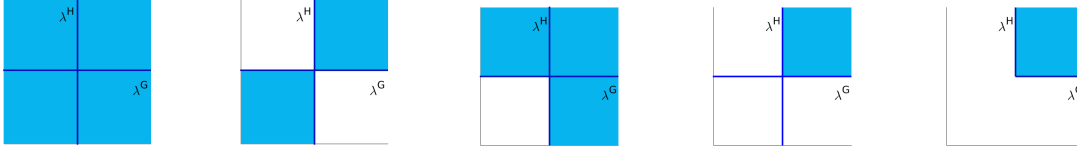
Figure 2: Signs of \lambda^G, \lambda^H for indices i \in \mathcal{I}^{00} . From the left to the right : weak-stationary, C-stationary, A-stationary, M-stationary and S-stationary.
