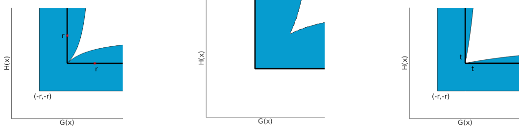
Figure 6: butterfly relaxations from left to right : B_{(t=r)} , B_{(s=t, 2t=r)} and B_{(t=r^{3/2})} .
