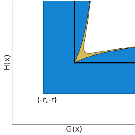
Figure 5: Feasible set of the butterfly relaxation with 2t = r and a constraint \Phi_i^B \leq \epsilon .
