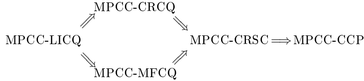
Figure 3: Relation between the MPCC-constraint qualifications
