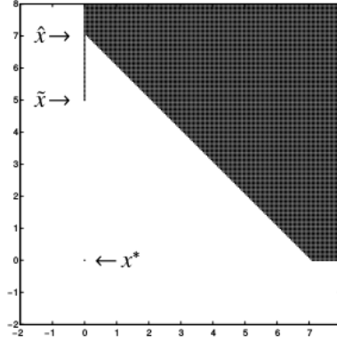
Figure 8: The feasible set of Example 5.3 from [37].
