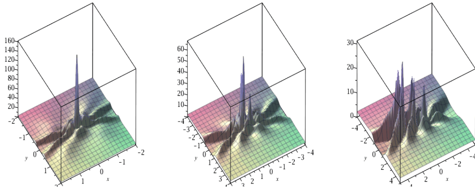
Figure 1. Solution of order 4 to KPI, on the left for t = 0 ; in the center for t = 0, 01 ; on the right for t = 0, 1 ; all the parameters to equal to 0.
