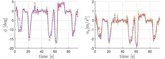
(a) Measured (blue) and estimated (red) roll angle
