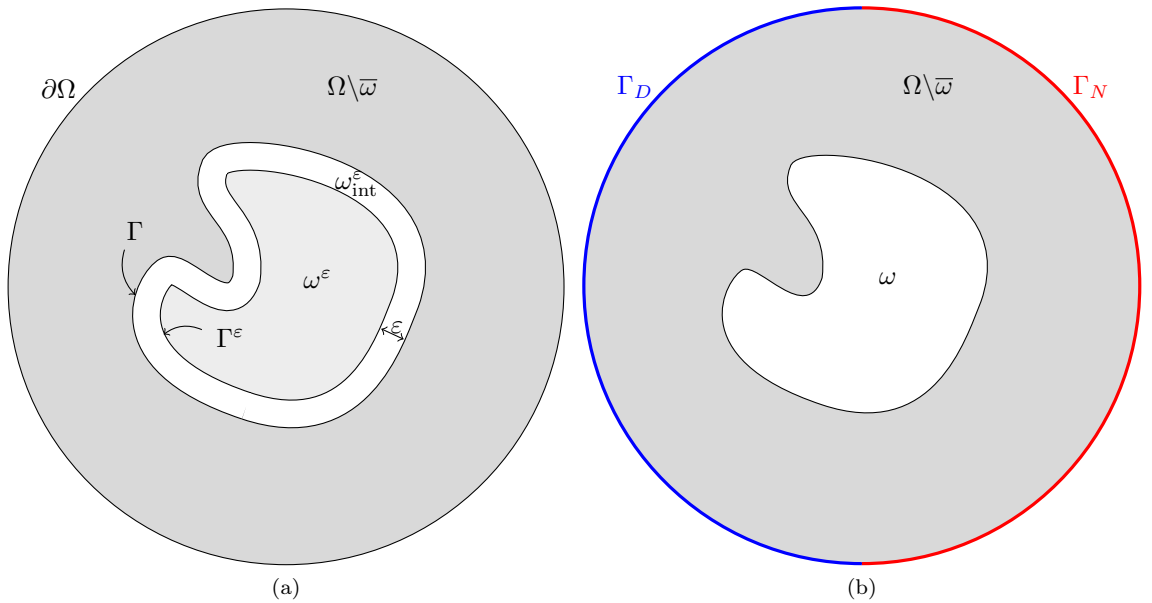
Figure 1: Notations for the thin layer model (left) and the obtained GIBC model (right).
