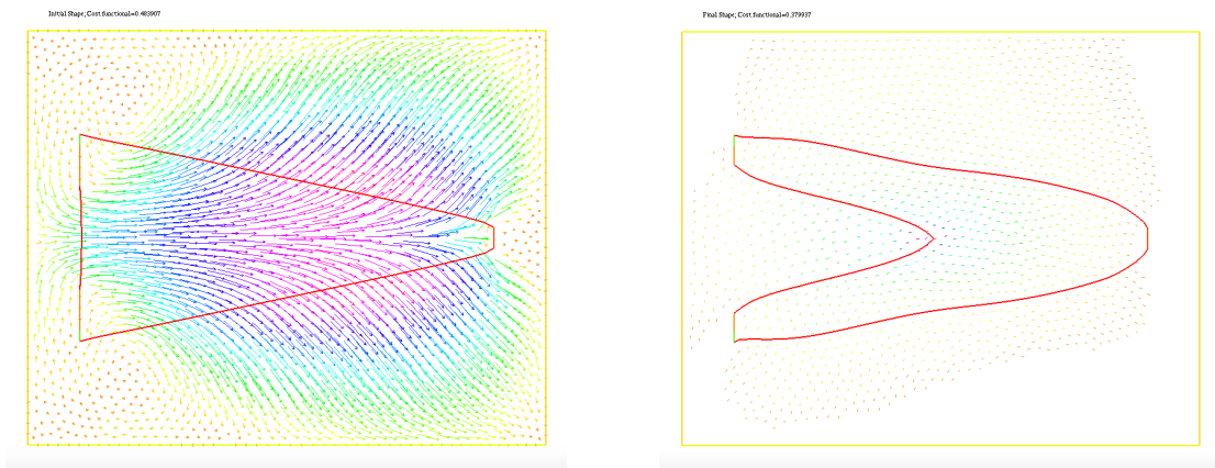
Figure 3: Minimization of the compliance for a 2d-cantilever: initial shape (left) and final shape (right).
