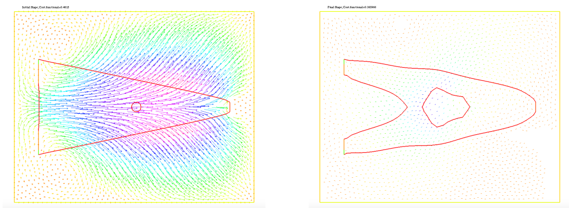
Figure 4: Minimization of the compliance for a 2d-cantilever with a hole: initial shape (left) and final shape (right).
