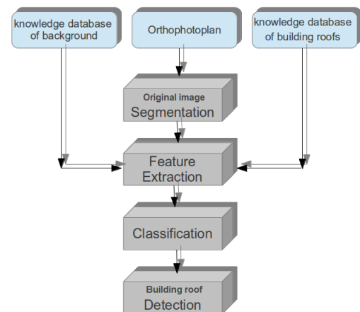
Fig. 2: General flowchart of the proposed building-detection method.
