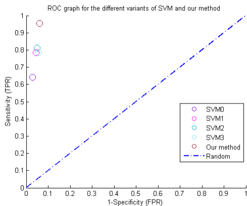
Fig. 10: The ROC graph comparing variants of SVM and the proposed method.
