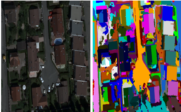
Fig. 3: Example of segmentation result using Statistical Region Merging (SRM) method. From left to right: Original image and its SRM segmentation result.
