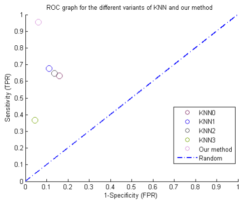
Fig. 9: The ROC graph comparing variants of KNN and the proposed method.
