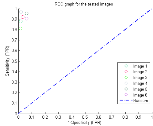
Fig. 6: The ROC graph of the test images using the proposed method.
