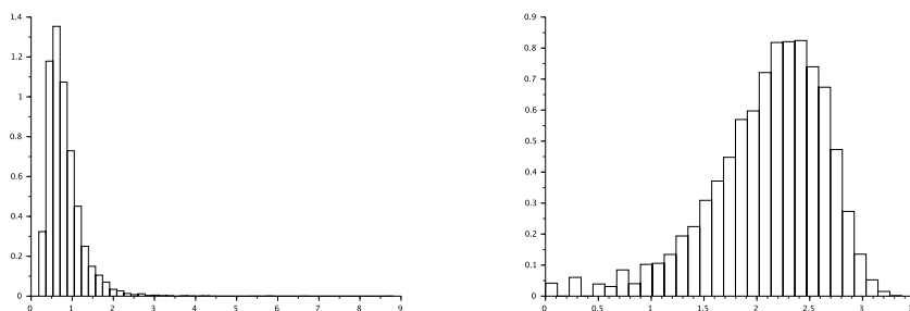
Figure 1: Histogram of the hitting time distribution for 10 000 simulations corresponding to the level L = 2 and starting position X_0 = 0 (left), histogram of the number of iterations in Algorithm (A1) in the \log_{10} -scale (right).
