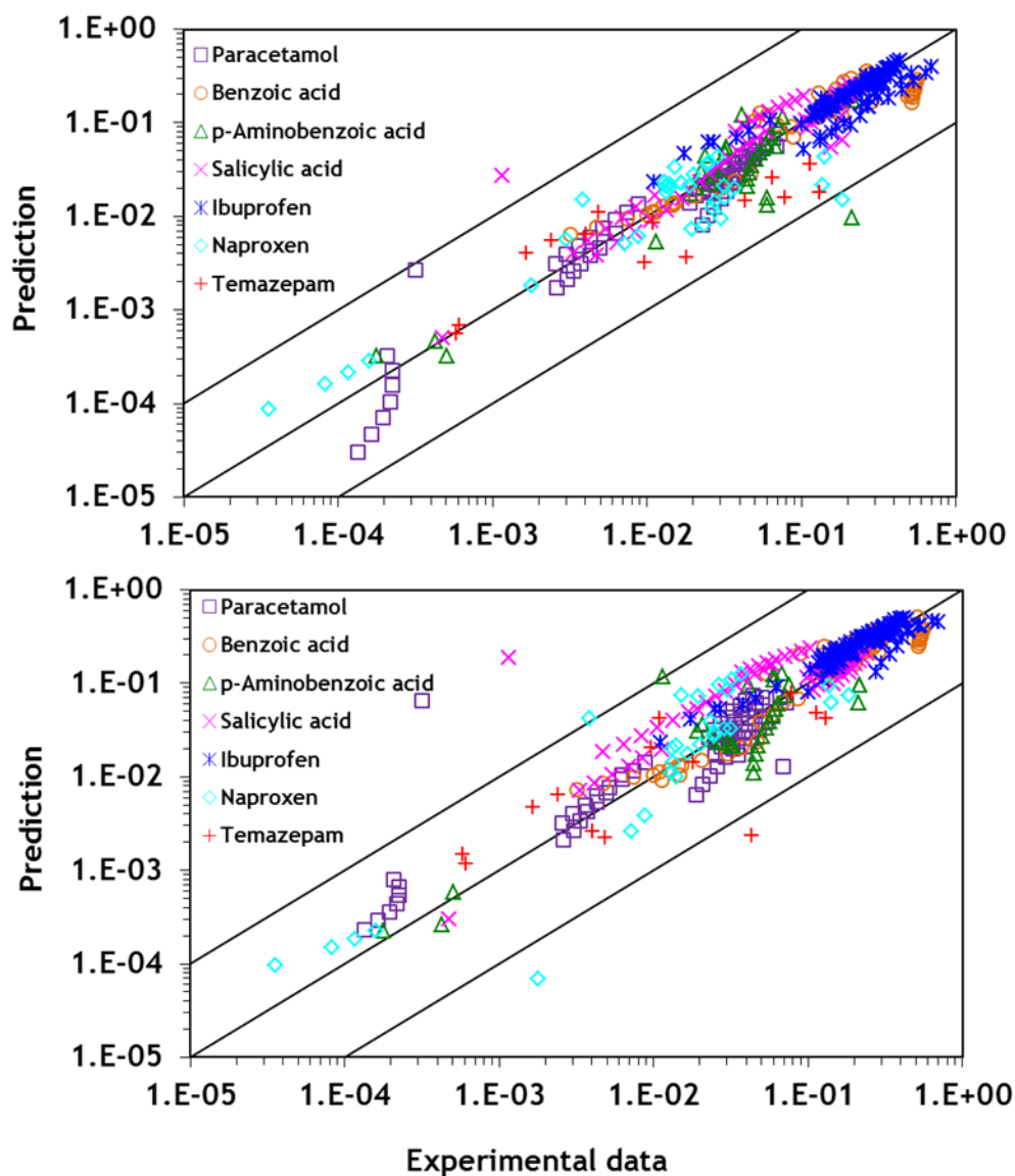
Figure 2 Predicted versus experimental solubility (mole fraction) of the pharmaceutical compounds in various pure solvents at one or more temperatures. Results with SciPharma (top) and NRTL-SAC (bottom).
