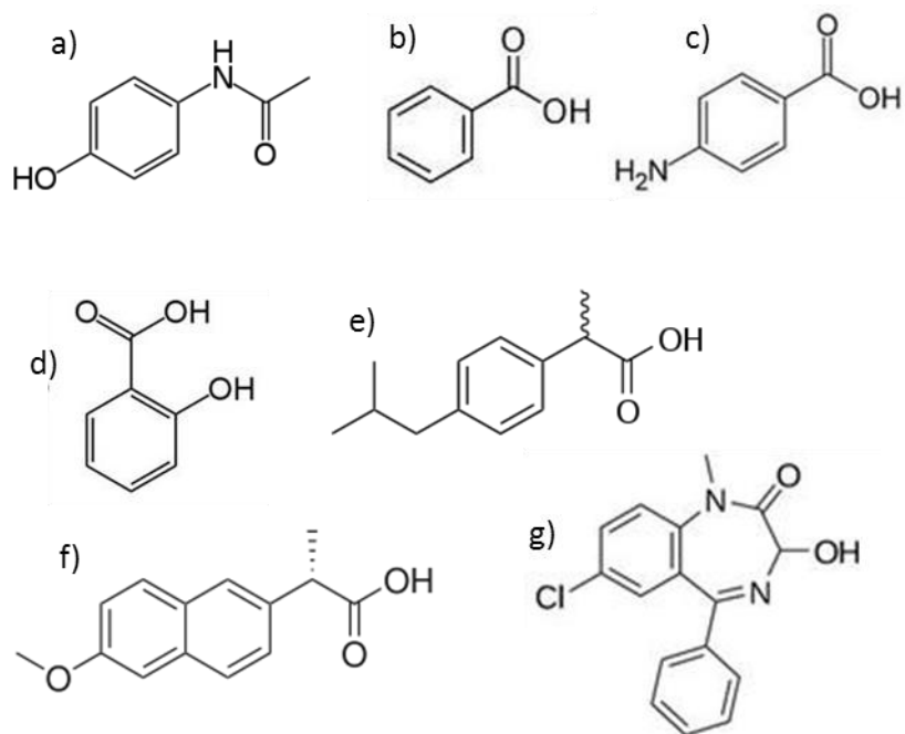
Figure 1 Chemical structure of the pharmaceuticals examined in this work: a) paracetamol, b) benzoic acid, c) p-aminobenzoic acid, d) salicylic acid, e) ibuprofen, f) naproxen and g) temazepam.
