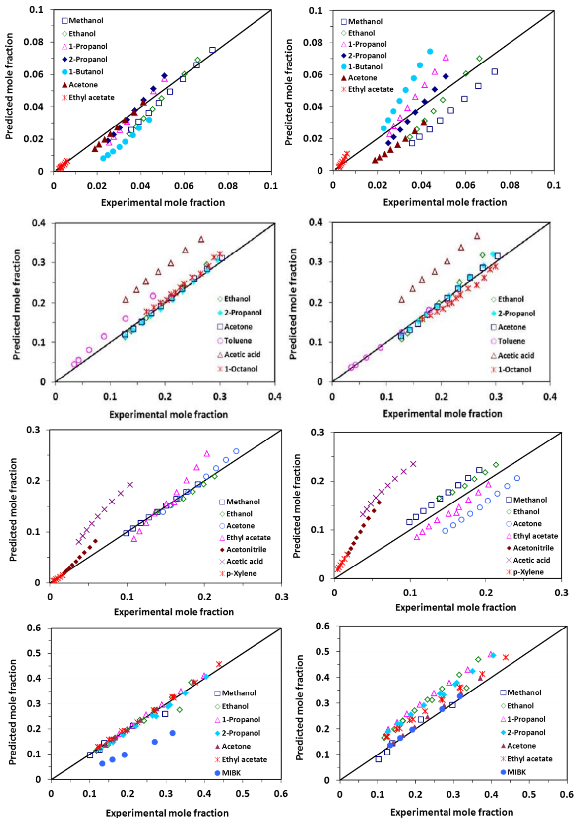
Figure 3 Predicted versus experimental solubility (mole fraction) for selected drugs in pure solvents at a range of temperatures to illustrate the temperature dependence of solubility. From top to bottom are shown: paracetamol, benzoic acid, salicylic acid, ibuprofen with SciPharma (left) and NRTL-SAC (right).
