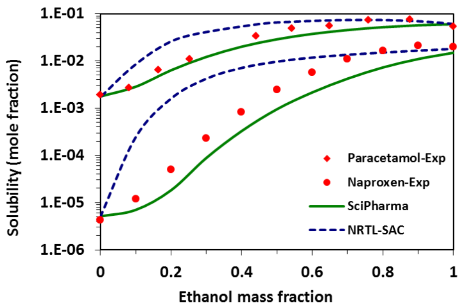
Figure 4 Experimental and predicted solubility of paracetamol and naproxen in the ethanol / water binary mixture at 298.15 K.
