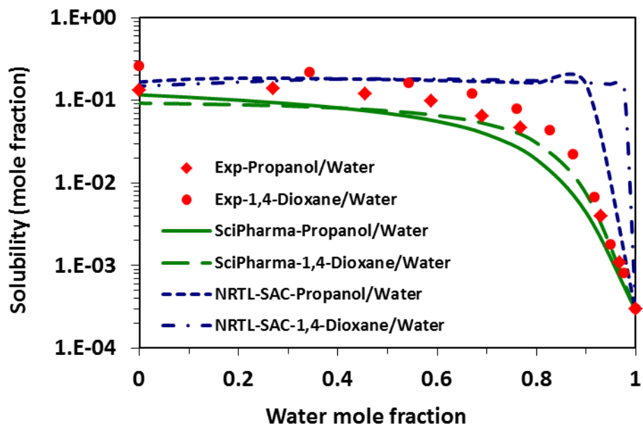
Figure 6 Experimental and predicted solubility of salicylic acid in the propanol / water and 1,4-dioxane / water mixtures at 298.15 K.
