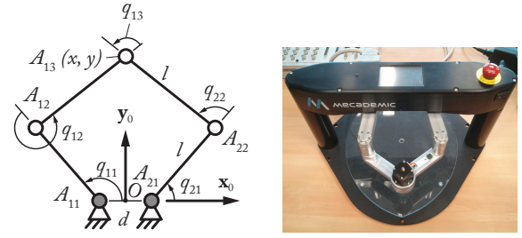
Figure 3: Five-bar mechanism and parametrization scheme
