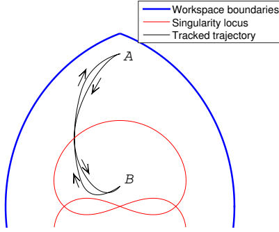
Figure 4: Tracked trajectory in Cartesian space (to scale)
