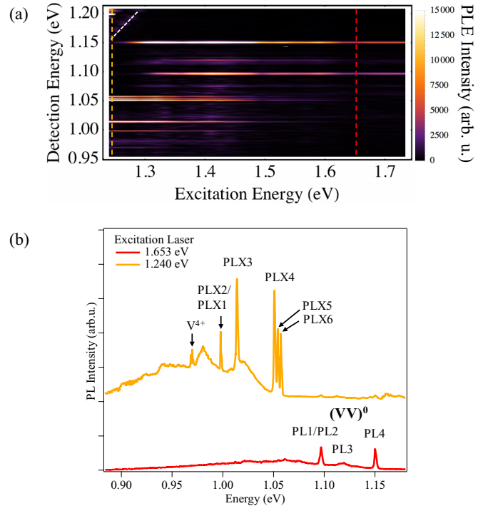
FIG. 2. Cryogenic temperature (10 K) PLE of a proton irradiated, high temperature annealed 4H -SiC sample. (a) PLE intensity map taken with 17 meV-increment excitation; broadband background (from phonon sidebands) was subtracted. The inclined dashed line is superimposed on the Raman LO line. (b) PL spectra at 1.653 eV and 1.240 eV excitation energies, indicated by vertical dashed lines in (a). In addition to the divacancy ZPLs (PL1–PL4), new ZPLs (PLX1–PLX6) are observed (vanadium-related ZPLs marked with V^{4+} ).
