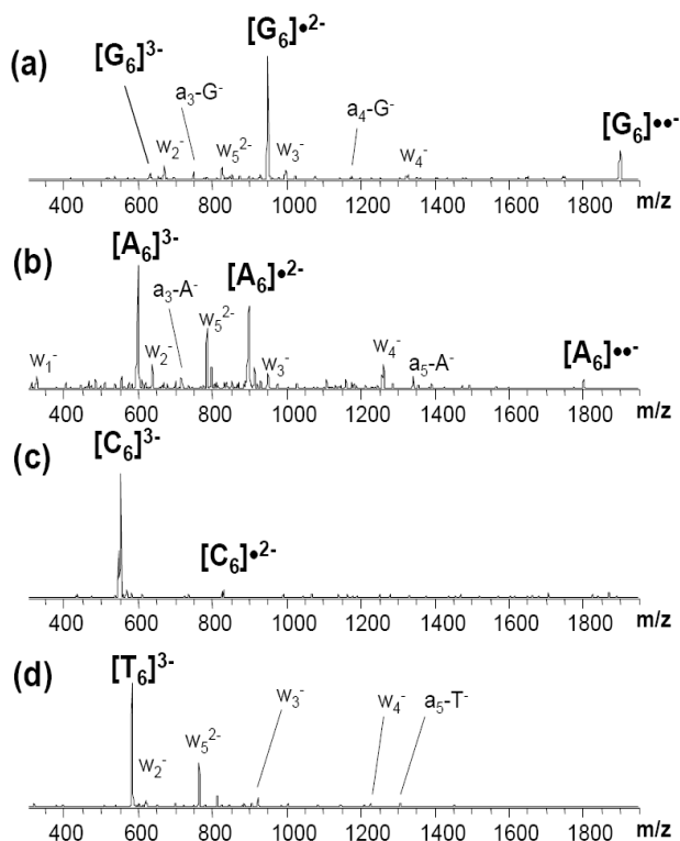
Figure 3. Electron photodetachment and secondary fragmentation as a function of the base: (a) [dG 6 ] 3- , (b) [dA 6 ] 3- , (c) [dC 6 ] 3- , (d) [dT 6 ] 3- . All [dB 6 ] 3- were isolated and subjected to 250 ms laser irradiation (5 laser pulses) at 260 nm, with identical laser focusing conditions and laser energy (fluence: 11.5 mJ/cm 2 ).
