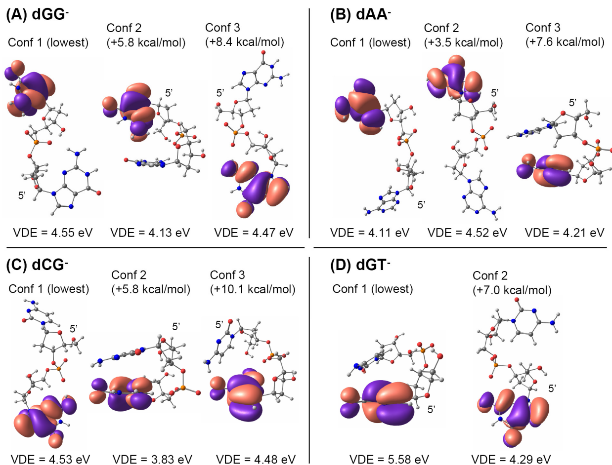
Figure 7. Relative energies (HF 6-31G+(d,p) + MP2 correction), HOMOs (HF 6-31G+(d,p)), and VDEs (HF 6-31G+(d,p) + MP2 correction) of different conformers of the deprotonated dinucleotides monophosphates (A) dGG - , (B) dAA - , (C) dCG - , and (D) dGT - .
