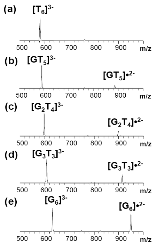
Figure 2. Electron photodetachment as a function of the guanine content: (a) [\text{dT}_6]^{3-} , (b) [\text{dGT}_5]^{3-} , (c) [\text{dG}_2\text{T}_4]^{3-} , (d) [\text{dG}_3\text{T}_3]^{3-} , and (e) [\text{dG}_6]^{3-} . All [6-mers] ^{3-} were isolated and subjected to a single 260-nm laser pulse, with identical laser focusing conditions and laser energy (fluence: 11.5 mJ/cm ^2 ).
