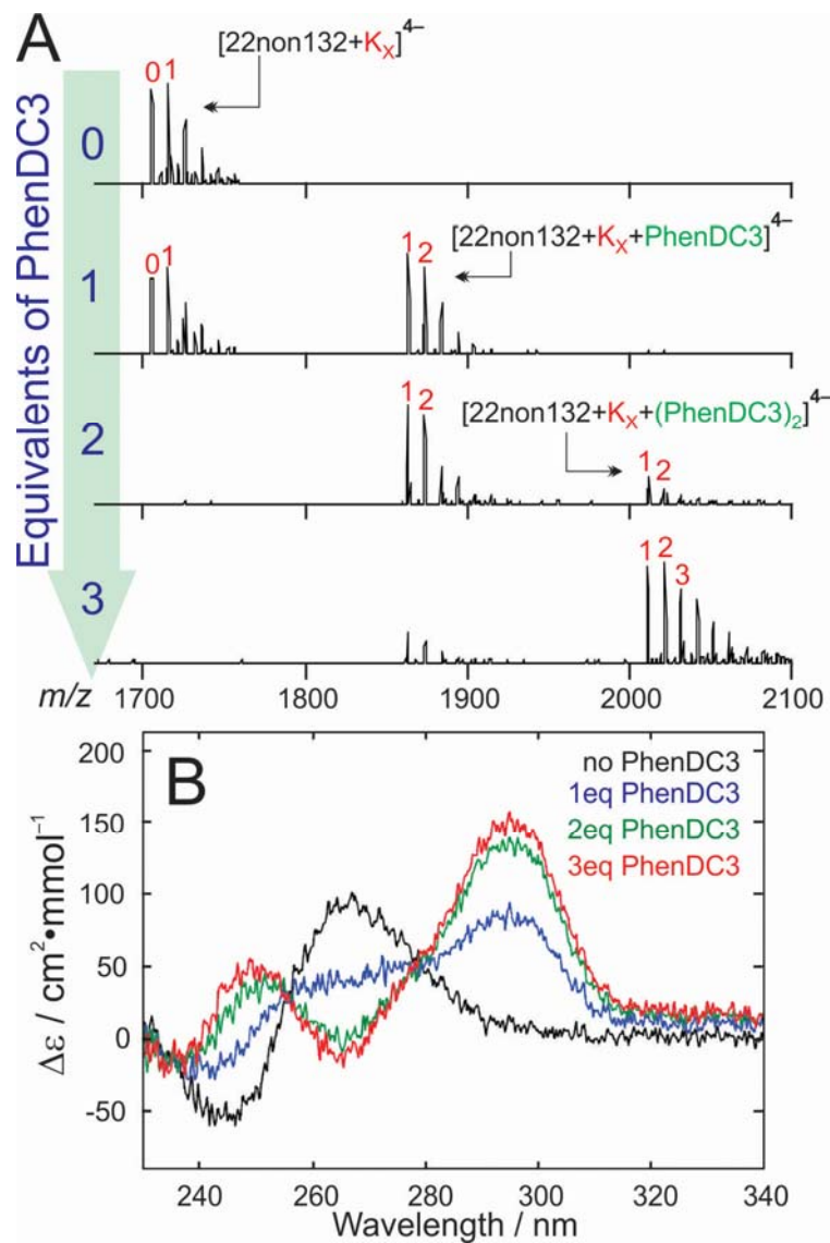
Figure 7. (A) Mass spectra of 5 \mu\text{M} 22non132 in the presence of 0, 1, 2 and 3 concentration equivalents of the ligand L = \text{PhenDC3} . Binding of one PhenDC3 ligand results in loss of a \text{K}^+ ion. (B) The circular dichroism (CD) spectra acquired for 5 \mu\text{M} 22non132 when combined with 0 – 3 equivalents of PhenDC3. The CD spectrum evolves from being representative of an unfolded oligonucleotide at low PhenDC3 concentration to being representative of an antiparallel G4 structure at high PhenDC3 concentration.
