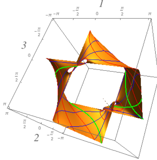
FIGURE 4. A slice \pi_+(\pi_-^{-1}(v)) of the scattering surface.
