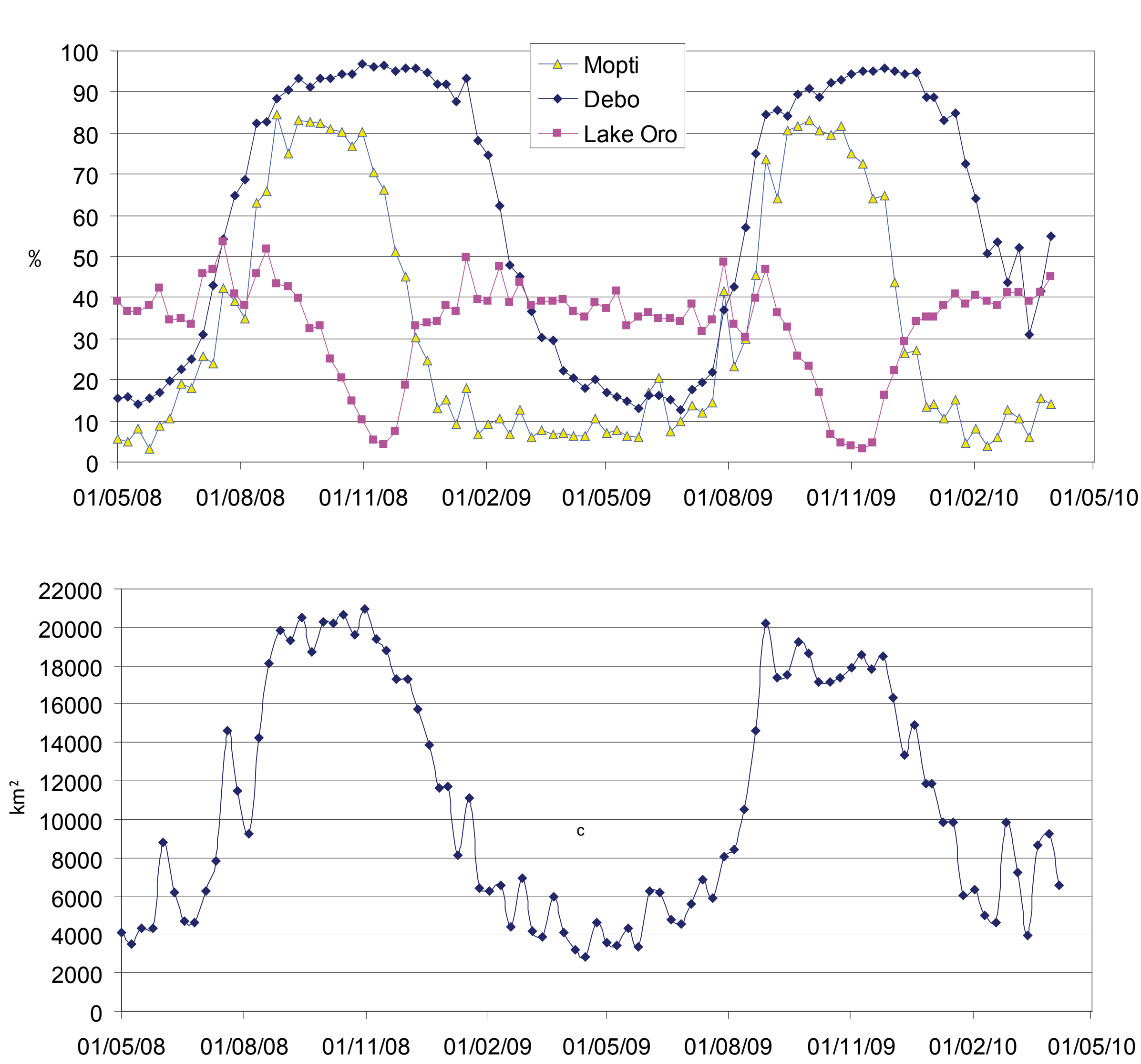
Fig. 6(upper): Variations in % of flooded area over 2008-2010 for 3 grid cells: Mopti on the Niger River, Lake Debo a central floodplain and Lake Oro in the North Fig. 6(lower): Variations in km² for the sum of the Inner Delta grid cells over 2008-2010
