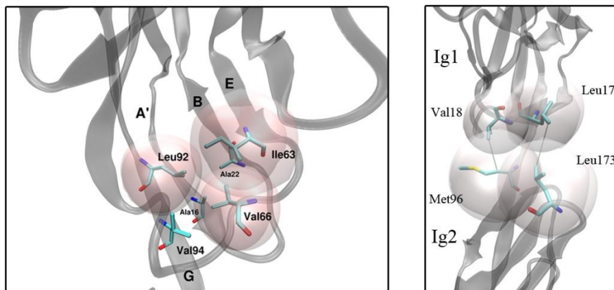
Fig. 3. Possible van der Waal interactions. The image was created using the VMD [28] analysis software.
