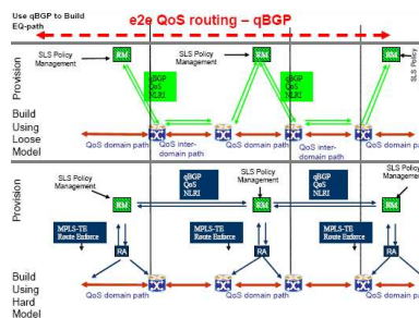
Fig. 4. Loose and hard forward models over multiple QoS domains
