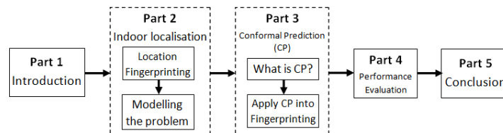
Fig. 1. Paper progression
