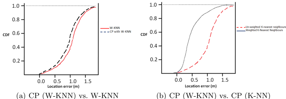
Fig. 5. Performance of CP with W-KNN and K-NN
