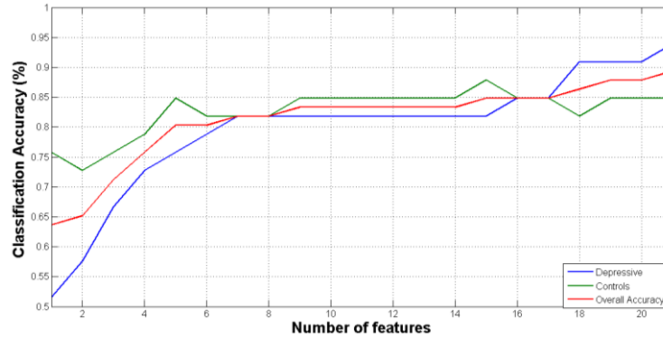
Figure 3 Classification accuracy of the Mahalanobis Distance (MD) based classifier.
