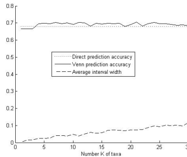
Fig. 2. Prediction accuracy and interval width for HD data for different K .
