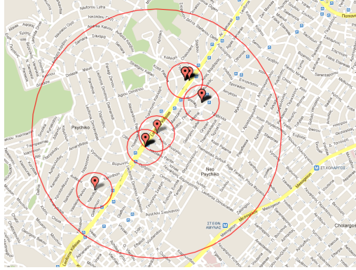
Fig. 2. A geo-cluster and all places extracted within it, using KVQ. Red markers mark photos. The radius of a geo-cluster is r_g = 700m , while the one of a place is r_p = 100m .
