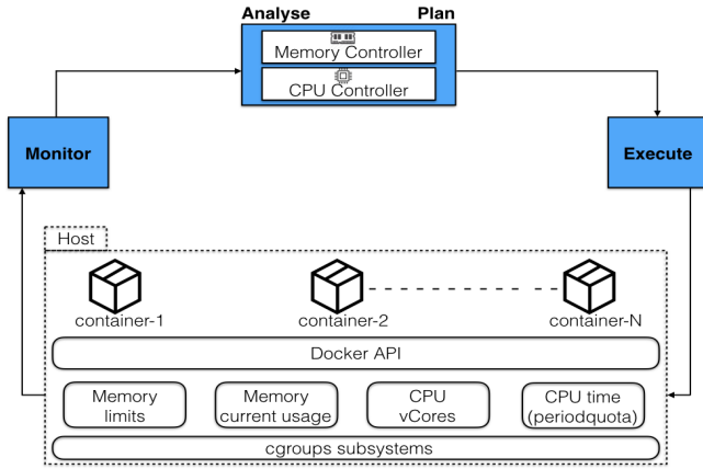
Fig. 2. ELASTICDOCKER architecture
