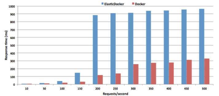
Fig. 4. Graylog response time with Docker vs ElasticDocker
