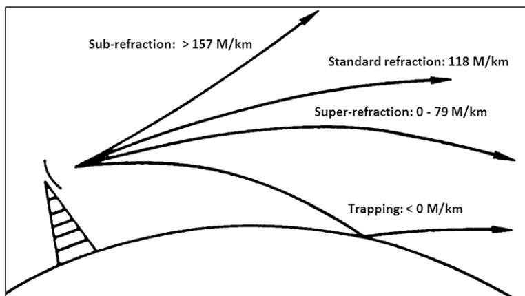
FIG. 1. Refraction of radio waves can be categorized as either sub-refractive, standard, superrefractive, or trapping, depending on the vertical gradient of the modified refractivity ( M units \text{km}^{-1} ) of the atmosphere.
