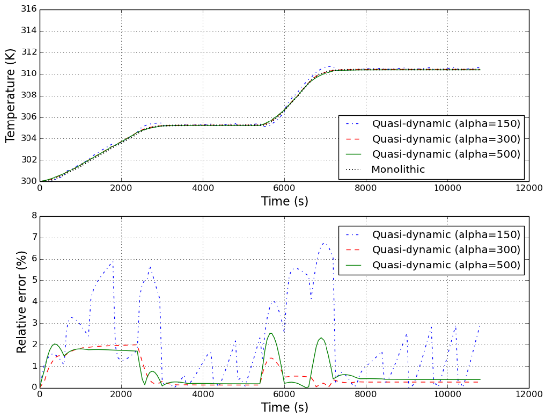
Figure 5: temporal evolution of temperature (above) and relative error (below) at point x=5cm of upper face, for coupling relaxation parameters \alpha = 150 , \alpha = 300 and \alpha = 500
