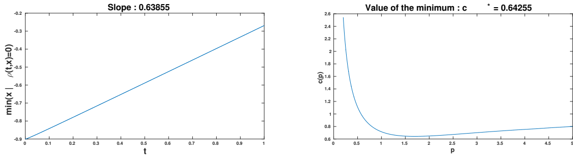
Figure 10: Left: The place of the front \min_x \{\rho(t, x) = 0\} as a function of t , computed with \Delta t = 3.125 \cdot 10^{-4} , \Delta x = 1.25 \cdot 10^{-3} and \Delta v = 1.25 \cdot 10^{-2} . The slope of the line gives the numerical propagation speed of the front. Right : The quantity c(p) (46) as a function of p . The theoretical front propagation speed is the minimal value of c(p) .
