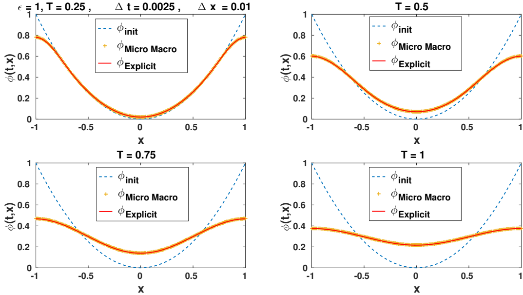
Figure 1: The solutions of (23) and (42) for \varepsilon = 1 at times T = 0.25, 0.5, 0.75, 1 , computed with \Delta t = 2.5 \cdot 10^{-3} , \Delta x = 10^{-2} and \Delta v = 1.25 \cdot 10^{-2} .
