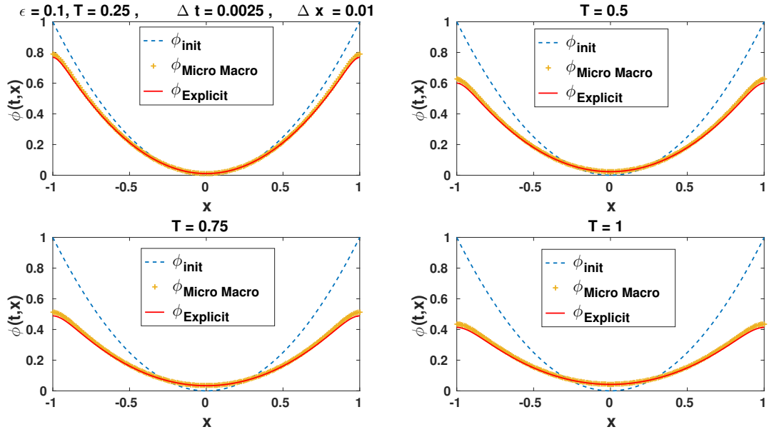
Figure 2: The solutions of (23) and (42) for \varepsilon = 10^{-1} at times T = 0.25, 0.5, 0.75, 1 , computed with \Delta t = 2.5 \cdot 10^{-3} , \Delta x = 10^{-2} and \Delta v = 1.25 \cdot 10^{-2} .
