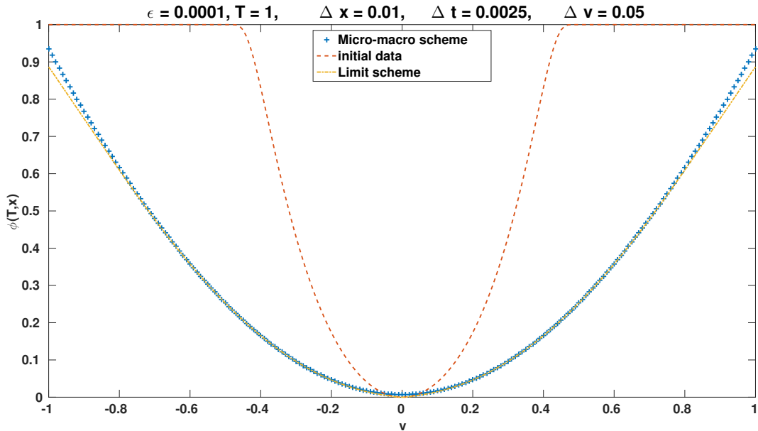
Figure 15: The Hopf-Cole transform of the density, \varphi , given by the micro-macro scheme and the limit scheme at time T = 1 , for \varepsilon = 10^{-4} , \Delta x = 10^{-2} , \Delta t = 2.5 \cdot 10^{-3} , \Delta v = 5 \cdot 10^{-2} .
