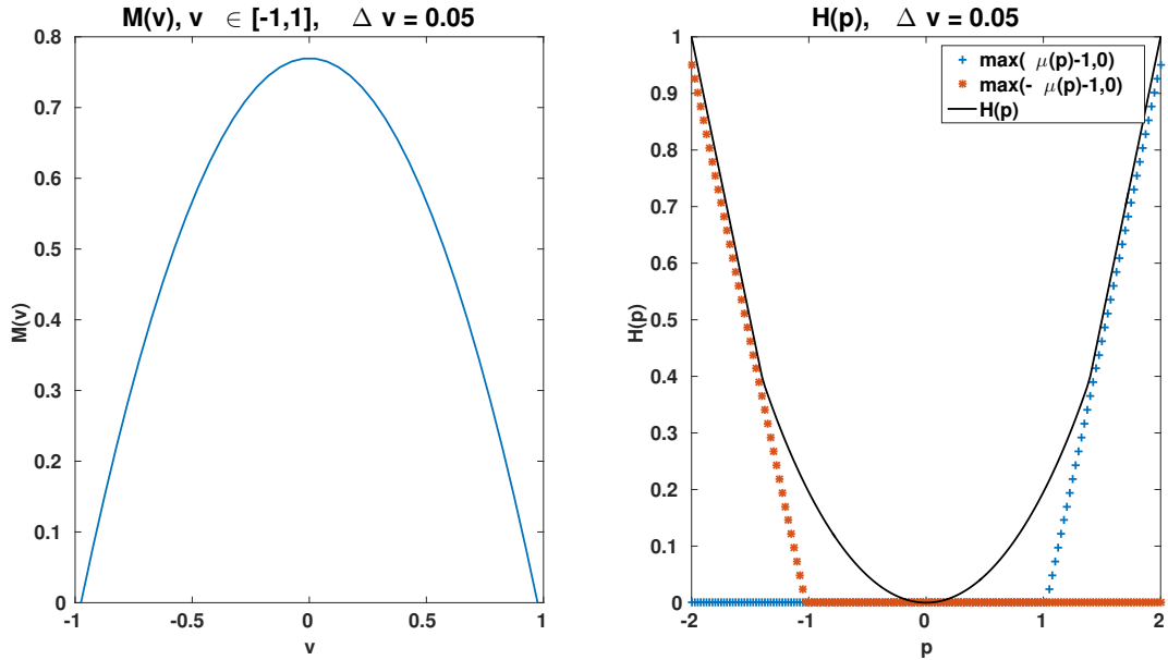
Figure 14: Left : The singular equilibrium considered in this section. Right : The constrained Hamiltonian H(p) computed with the limit scheme.
