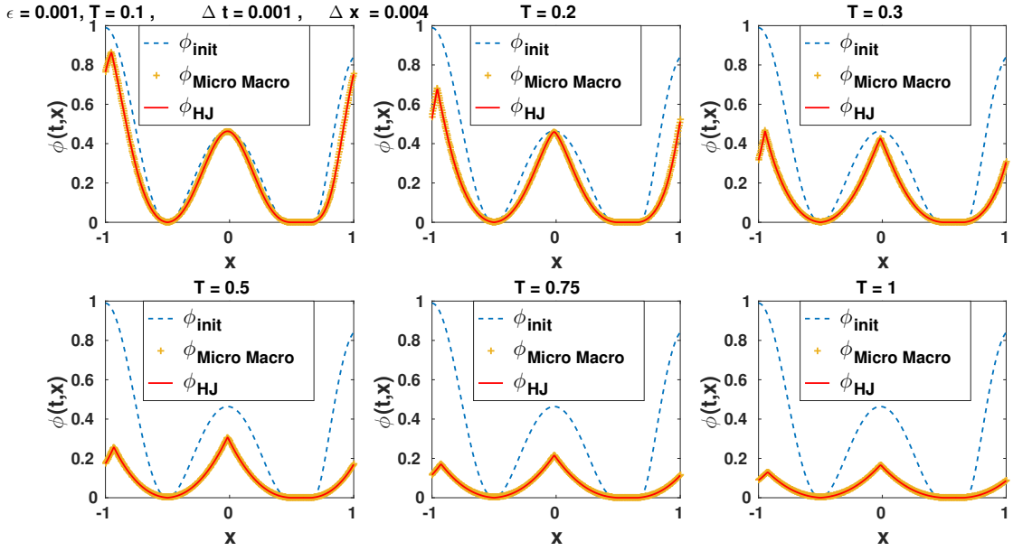
Figure 7: The solutions of (23) and (26) for \varepsilon = 10^{-3} at times T = 0.1, 0.2, 0.3, 0.5, 0.75, 1 , computed with \Delta t = 10^{-3}, \Delta x = 4 \cdot 10^{-3} and \Delta v = 1.25 \cdot 10^{-2} .
