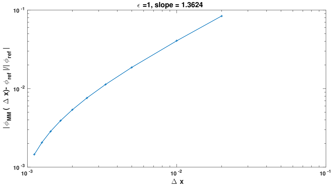
Figure 12: The expression E(1, \Delta x) in function of \Delta x (log scale).
