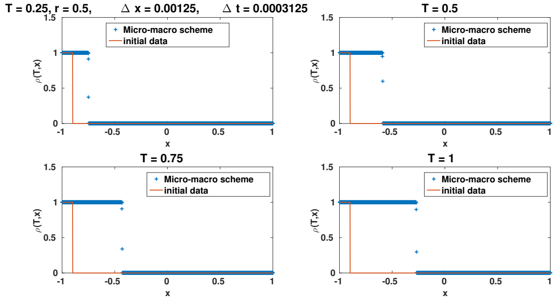
Figure 9: The solution of the micro-macro scheme (23) for \varepsilon = 10^{-4} at times T = 0.25, 0.5, 0.75 and 1, computed with \Delta t = 3.125 \cdot 10^{-4} , \Delta x = 1.25 \cdot 10^{-3} and \Delta v = 1.25 \cdot 10^{-2} .
