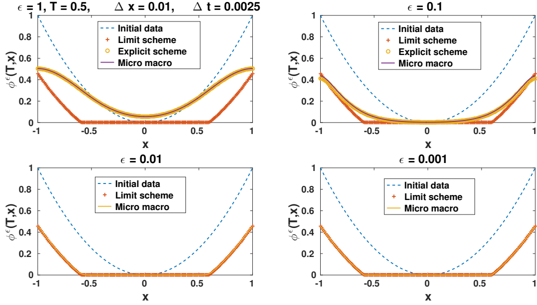
Figure 8: The solutions of (23), (42), and (26) for some values of \varepsilon at time T = 0.5 , computed with \Delta t = 2.5 \cdot 10^{-3} , \Delta x = \cdot 10^{-2} and \Delta v = 1.25 \cdot 10^{-2} .
