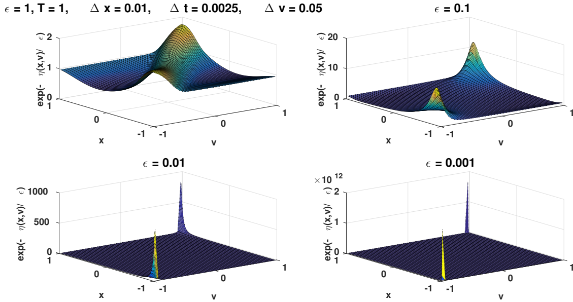
Figure 16: The corrector e^{-\eta^\epsilon(T,x,v)/\epsilon} given by the micro-macro scheme at time T = 1 , for different values of \epsilon , and \Delta x = 10^{-2} , \Delta t = 2.5 \cdot 10^{-3} , \Delta v = 5 \cdot 10^{-2} as a function of x and v .
