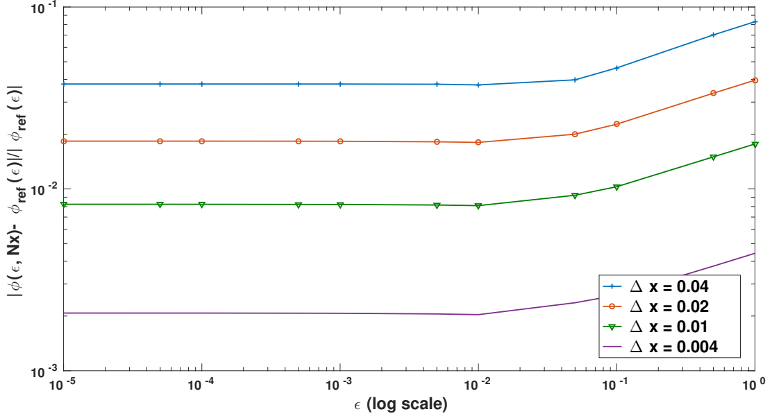
Figure 13: The expression E(\varepsilon, \Delta x) in function of \varepsilon for different values of \Delta x (log scale).
