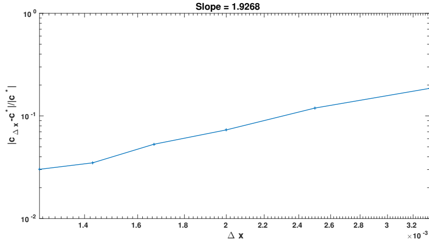
Figure 11: The relative error |c_{\Delta x} - c^*|/|c^*| as a function of \Delta x (log scale).
